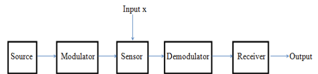
Figure 2: A fiber optic sensor system
