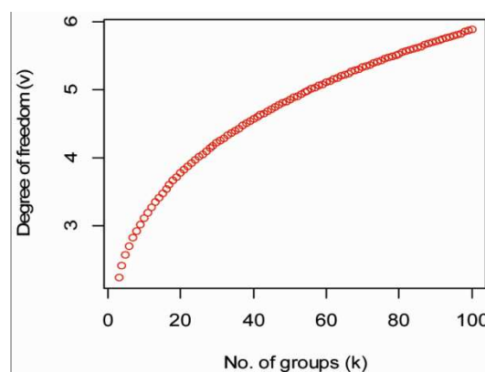
FIGURE 3: Graph of the plot of number of group ( k ) against empirical degree of freedom ( \nu ) for the proposed chi-squared distributed test statistic X_{max}^2 for comparing ordered population proportions with a control.
