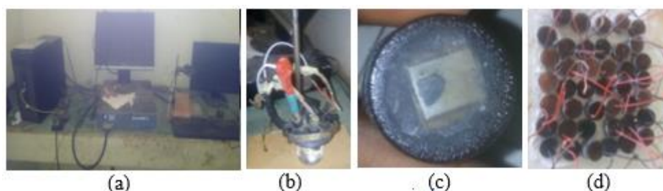
Fig. 3: (a) Electrochemical measurement analysis setup, (b) Connection of electrodes inside the medium, (c) mounted Tafel sample before polishing (d) Tafel samples ready for test
