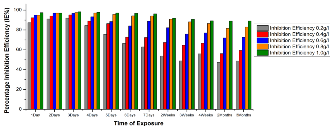
Fig. 6: Inhibition efficiency of Prosopis Africana pod extract (PAPE) on the corrosion of mild steel in 1M HCl solutions
