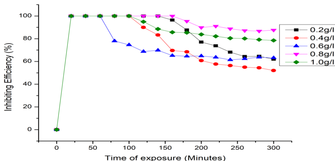
Fig. 8: Variation of inhibition efficiency vs. time of exposure of PAPE concentrations
