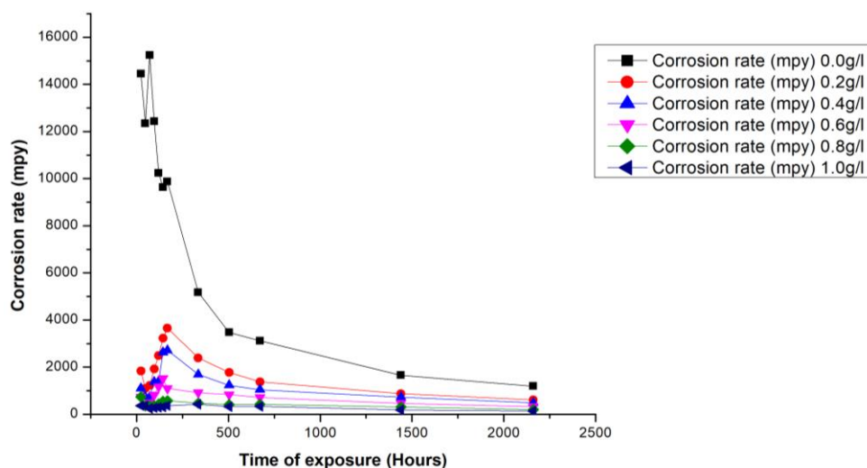
Fig. 5: Corrosion rate (mpy) against time (hours) of mild steel in 1M HCl with and without (0.0g/l) PAPE as inhibitor after 2160 hours of exposure
