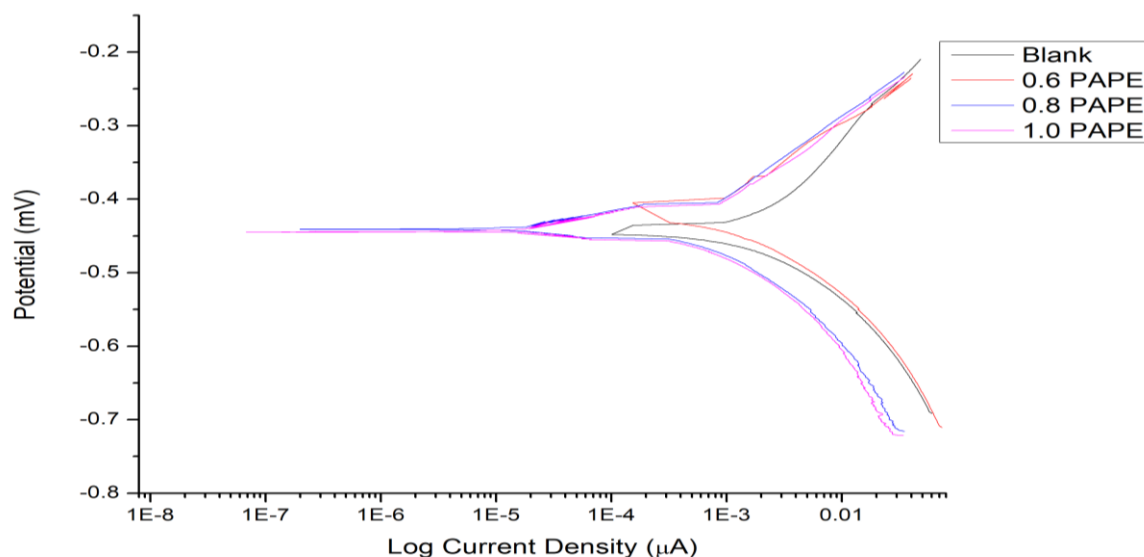
Fig. 9: Polarization curves of mild steel in 1M HCl with and without PAPE Inhibitor
