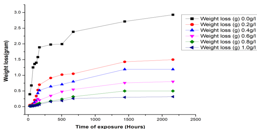
Fig. 4: Weight loss against time of mild steel in 1M HCl with PAPE inhibitor and without PAPE (0.0g/l) after 2160 hours of exposure
