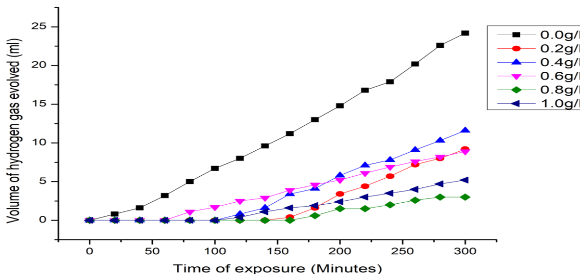
Fig. 7: Evolution rate of hydrogen gas in the acidic medium with PAPE concentrate
