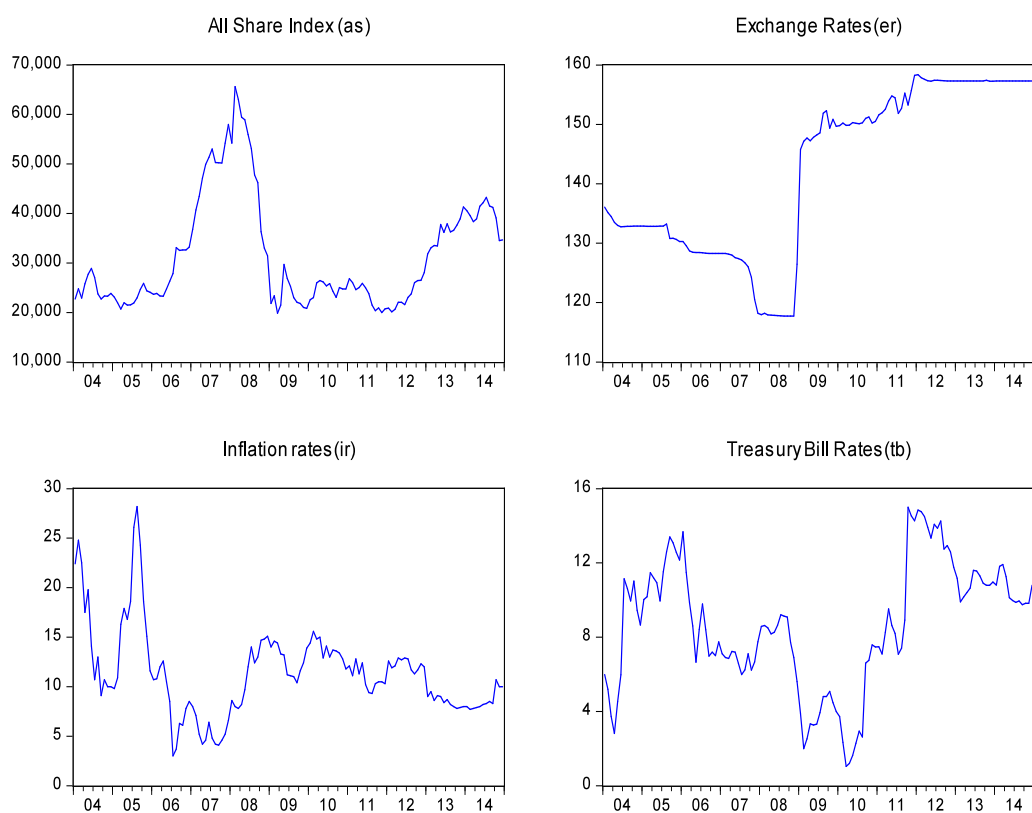
Figure 1. Time Plots on NSE All-Share Index, Nominal Exchange rate, Inflation rate and Treasury Bill rate (2004-2014)
