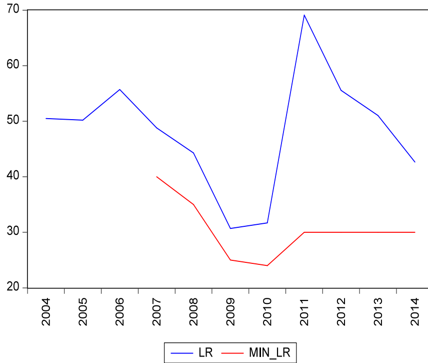
Figure 3. Banking Industry Liquidity Ratio (2004-2014)
