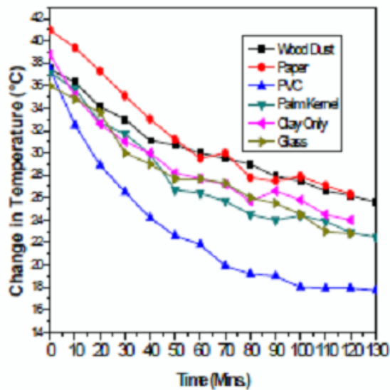
Fig. 1: Change in Temperature against the Time for particulate insulated Composite bricks
