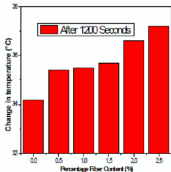
Figure 4: Change in Temperature against the Percentage Fiber Content
