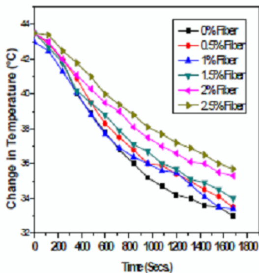
Fig. 3: Change in Temperature against Time for Fiber-Clay composite bricks
