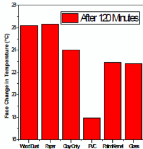
Fig. 2: Face Change in temperature against the Materials used after 120 Minutes
