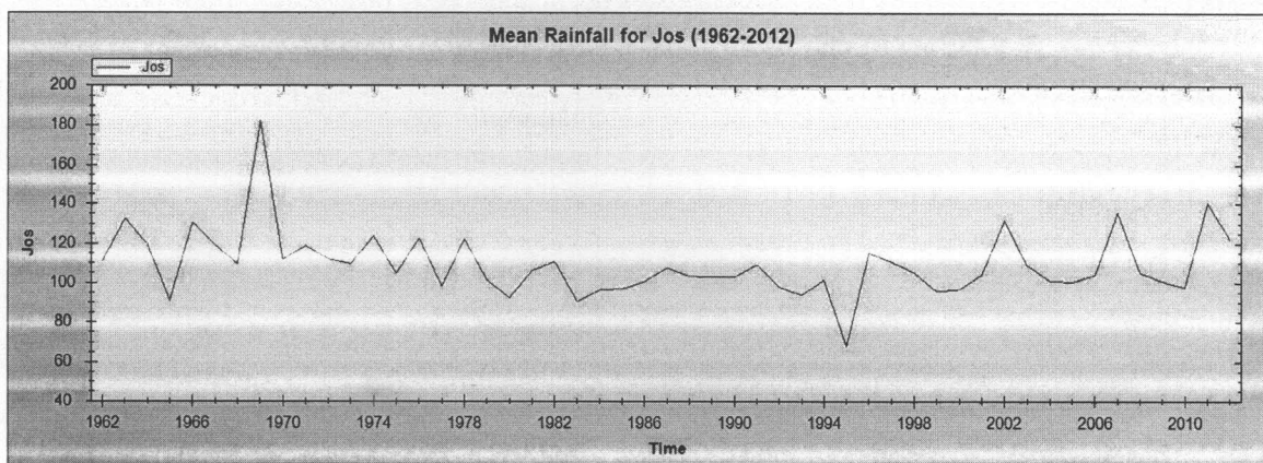
Figure 4: Normal Mean Distribution of Rainfall for Jos (1962-2012).
