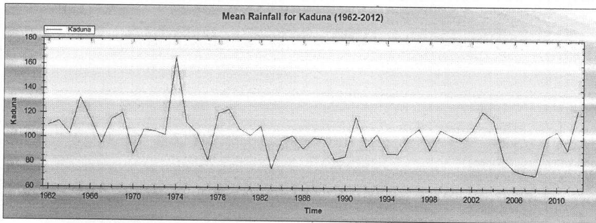
Figure 5: Normal Mean Distribution of Rainfall for Kaduna (1962-2012).
