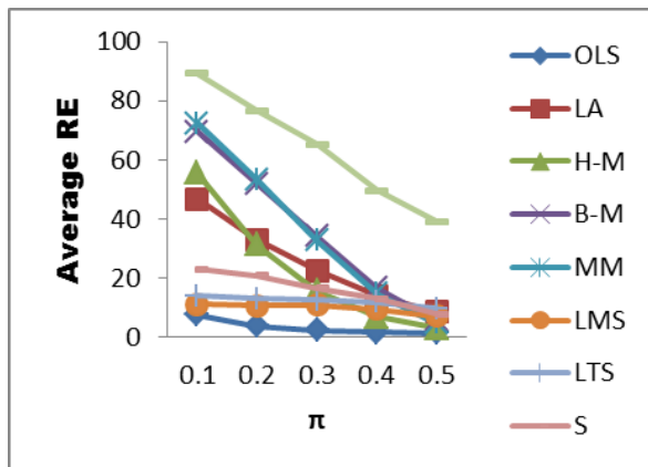
Figure 2: Plot of Average RE against Outlier Percentages for Case I.
