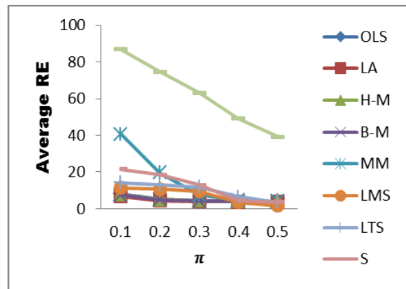
Figure 4: Plot of Average RE against Outlier Percentages for Case II.
