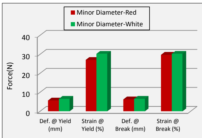
Figure 1: Kernel compression test-minor axis.
