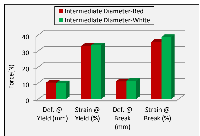
Figure 2: Kernel compression test-intermediate axis.
