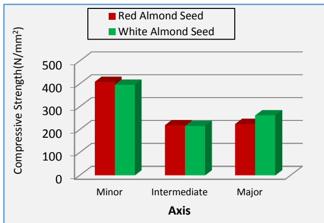
Figure 3: Comparing compressive strength at various axes.
