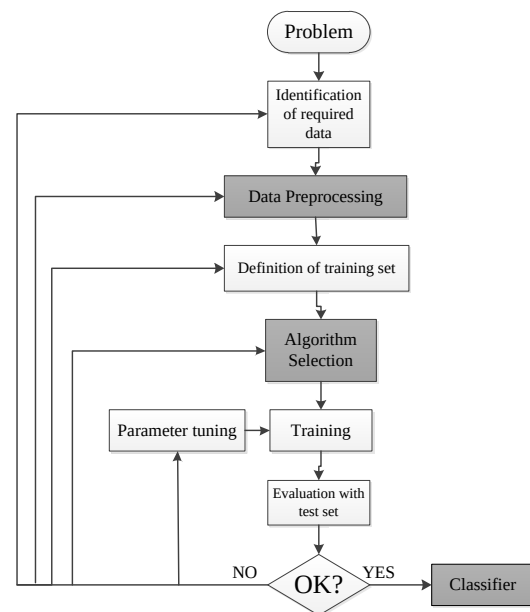
Fig 1: Text classification process (Kotsiantis, 2007).
