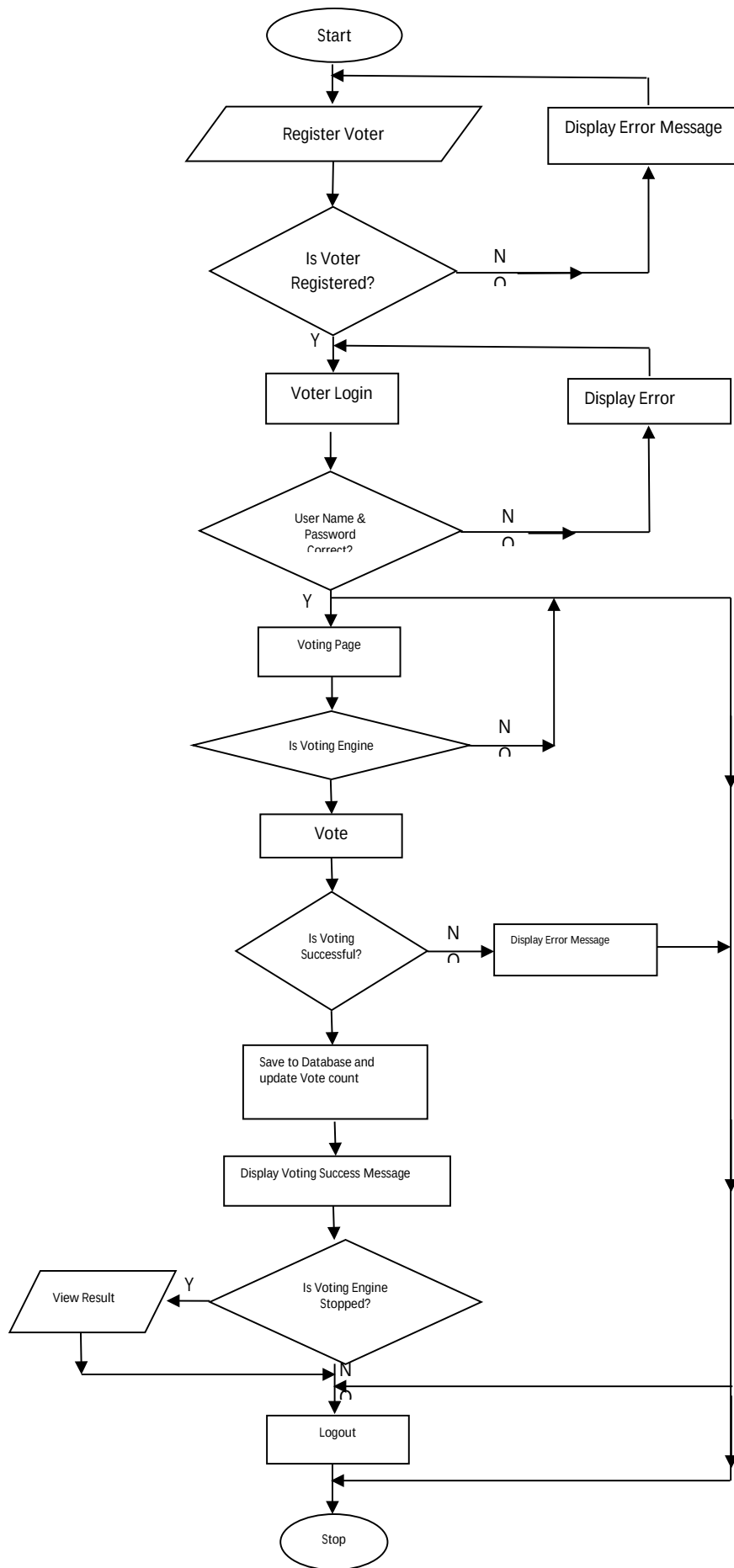
Figure 4: Application Flowchart
