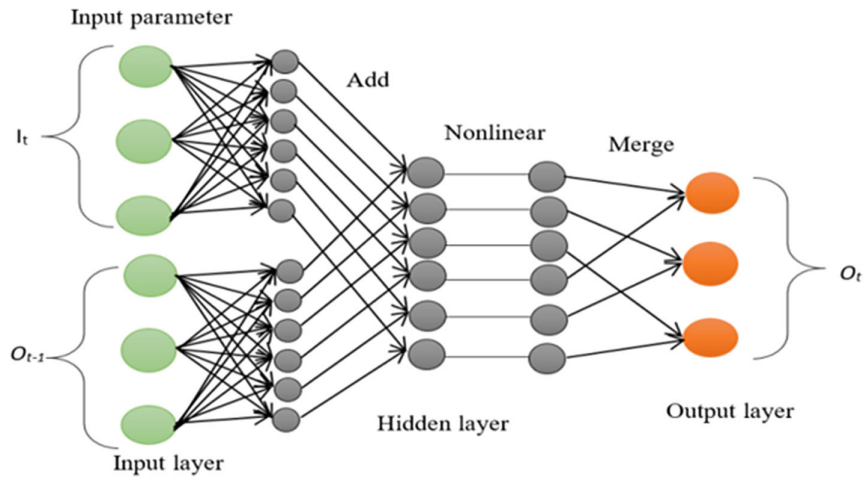
Figure 7 Basic structure of RNN architecture
