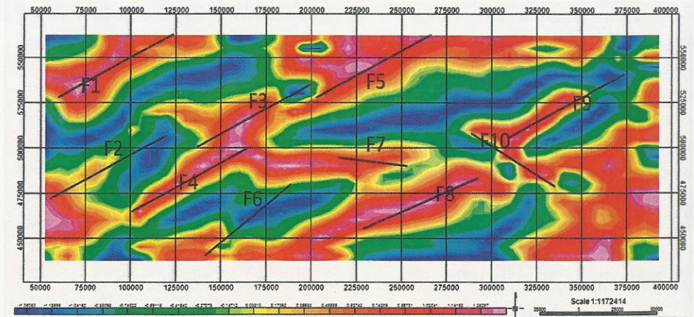
Fig. 6c: Tilt angle map of the study area
