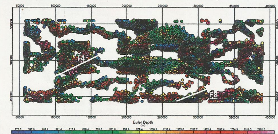
Fig. 8a Euler depth slice for solutions between 0-3 km
