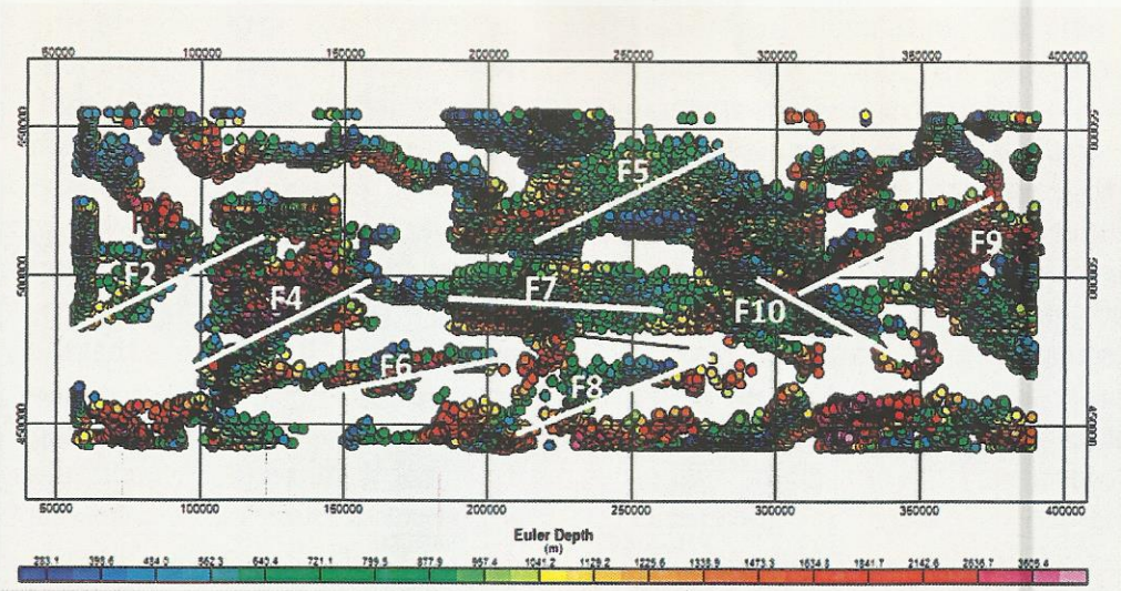
Fig. 6d: Euler Deconvolution (for all solutions) Map of the study area
