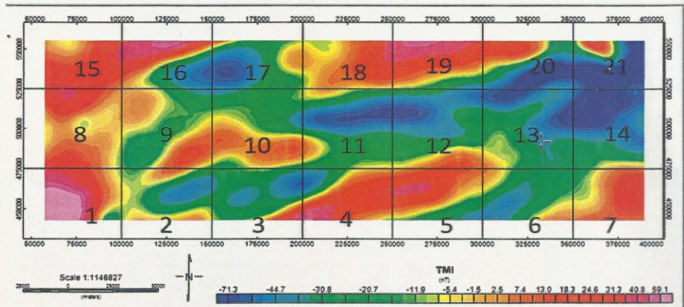
Fig. 5b: TMI map showing the division of the study area into 21 blocks
