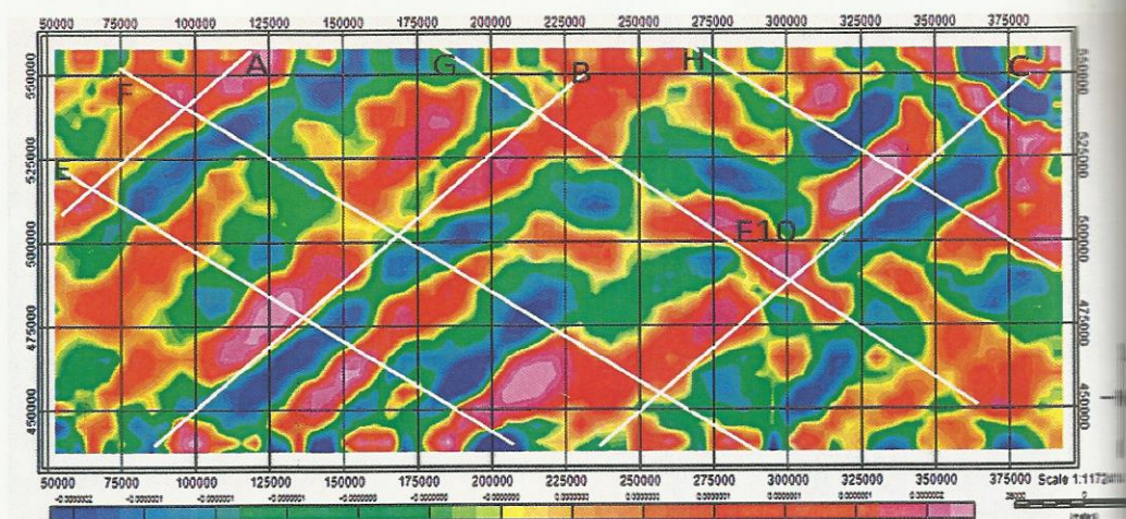
Fig.9: Second Vertical Derivative Map
