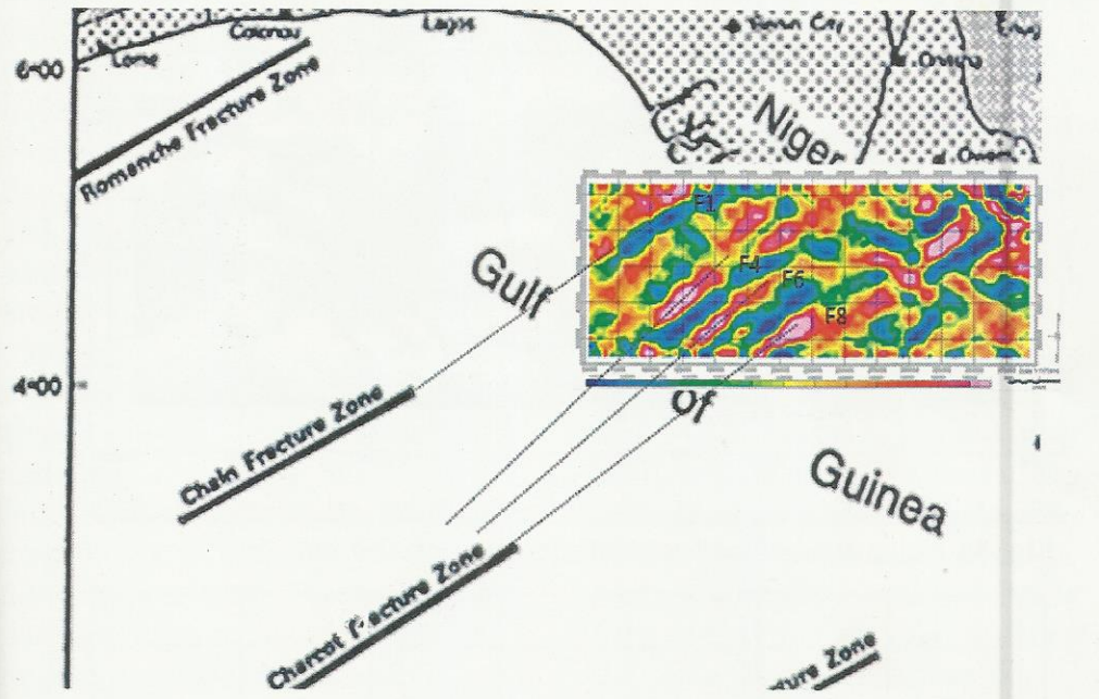
Fig. 6d: Euler Deconvolution (for all solutions) Map of the study area
