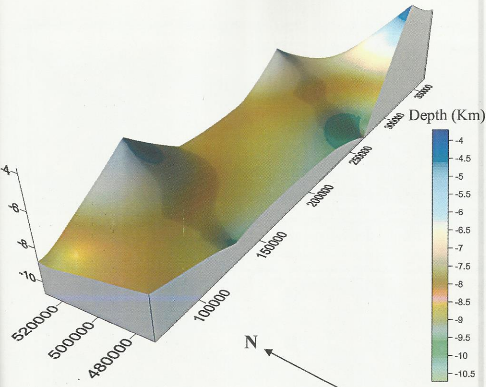
Fig. 5c: 3-D basement topography of the study area
