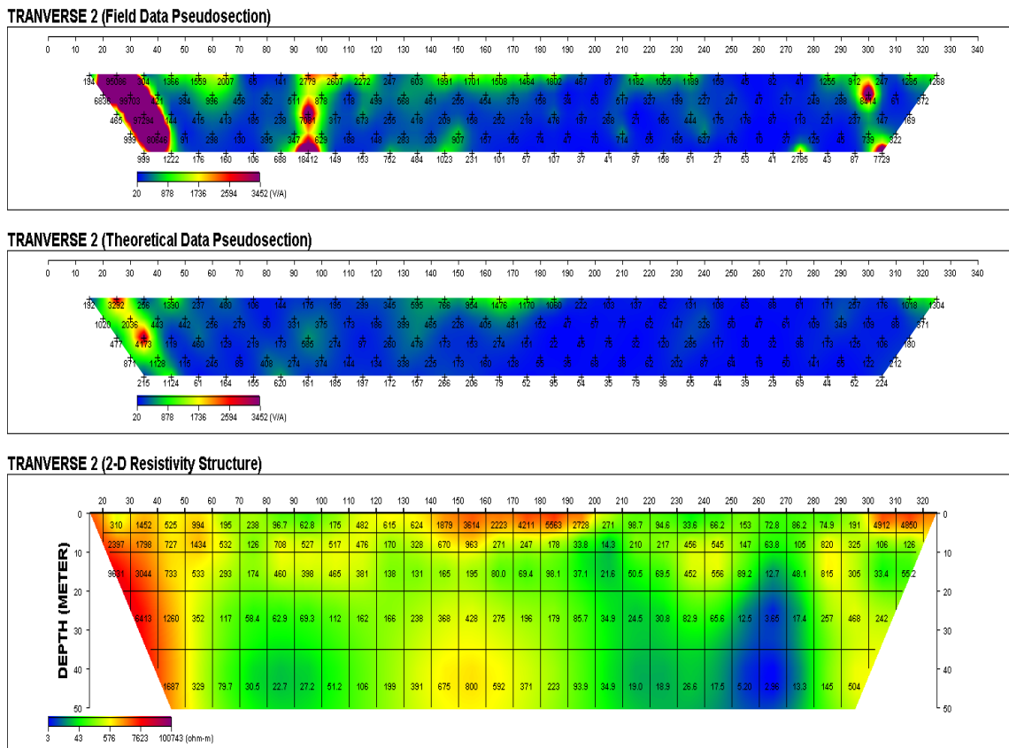
Figure 8: Interpreted geo-electrical section of RTM 2 profile of Asa earth embankment
