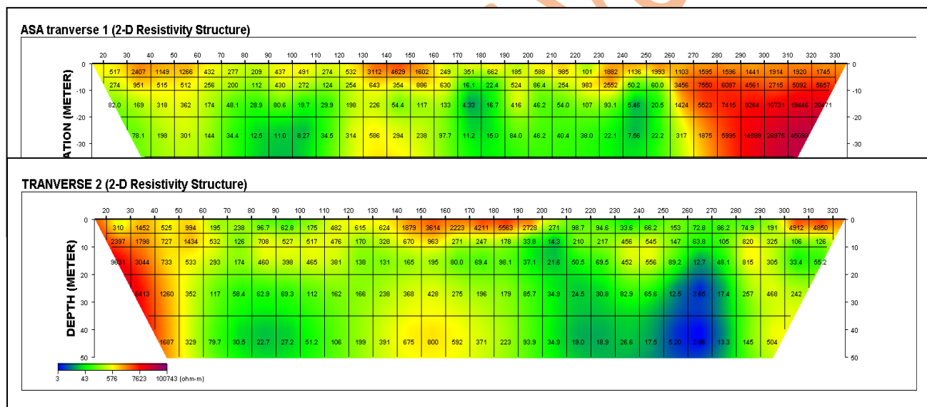
Figure 9 Correlation of RTM1 and RTM2 of Asa earthdam embankment
