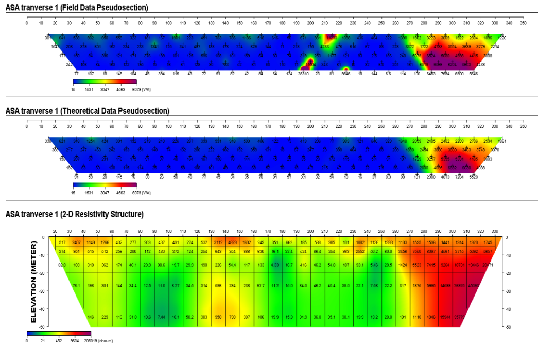
Figure 7: Interpreted geo-electrical section of RTM 1 profile of Asa earthembankment
