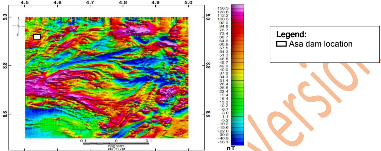
Figure 4: The Reduced to pole map of sheet 202
