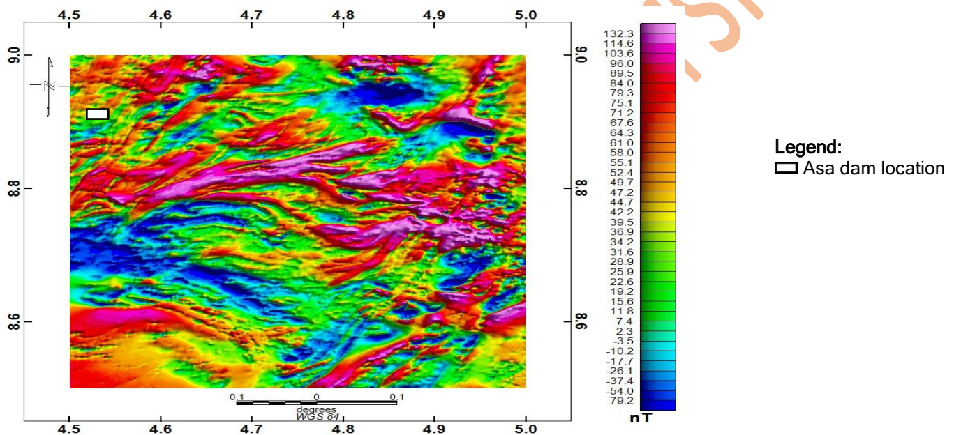
Figure 3: The Residual Magnetic Intensity map of sheet 202
