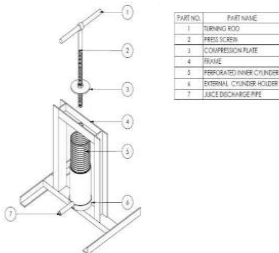
Fig. 1: Part List of the Machine
