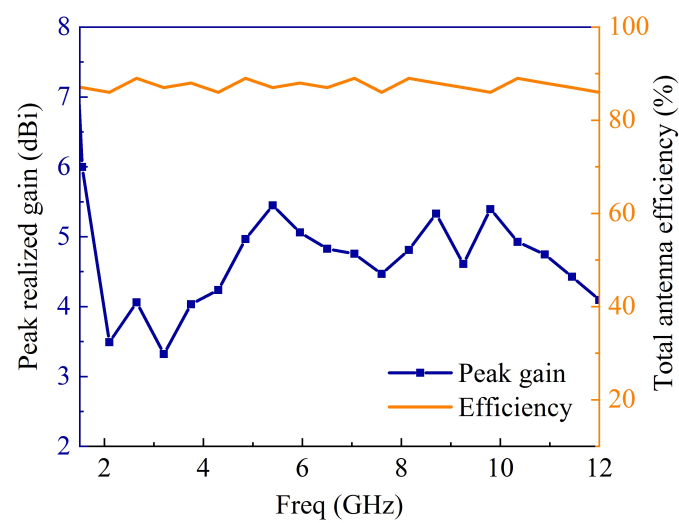
Figure 25. Antenna peak gain and efficiency.
