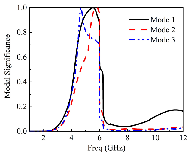
Figure 12. Modal significance at 5.5 GHz.
