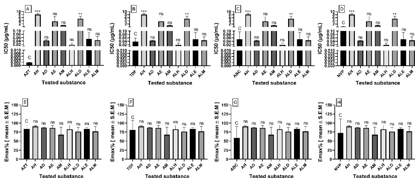
Figure 3. IC 50 (A, B, C and D) and Emax (E, F, G and H) values of the control drugs and the tested fractions antiviral activity. Results expressed are mean of three independent experiments \pm S.E.M. C; control, ns; not significant, **, P < 0.01 , ***, P < 0.001 . AZT= Zidovudine; TDF= Tenofovir; ABC= Abacavir; NVP= Nevirapine; AH= hexane fraction of the bark; AD= dichloromethane fraction of the bark; AM= methanol fraction of the bark; AE= Ethyl acetate fraction of the bark; ALH= hexane fraction of the leaves; ALD= Dichloromethane fraction of the leaves; ALE= ethyl acetate fraction of the leaves; ALM= methanol fraction of the leaves.
