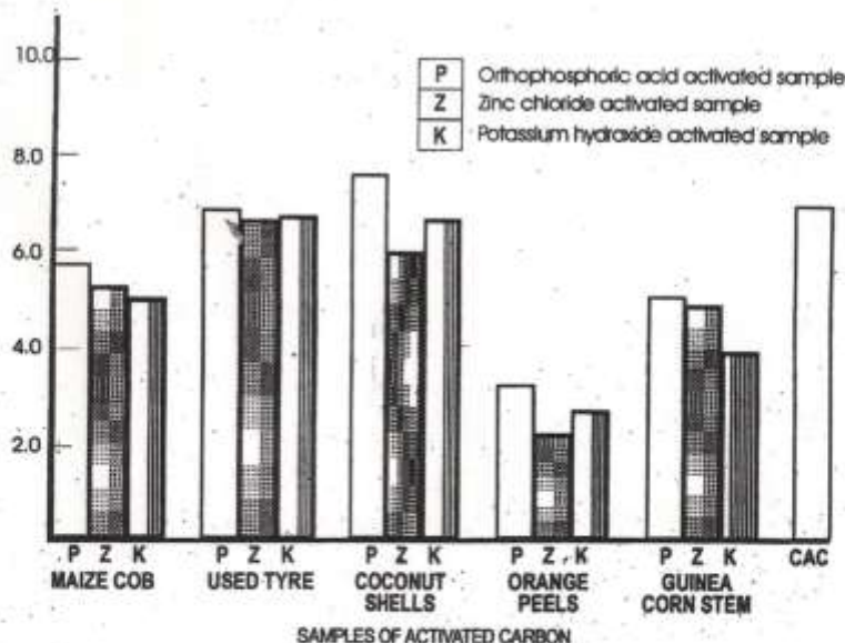
Fig. 1: Adsorption capacity of activated carbon based on decolorisation of methylene blue solution.
