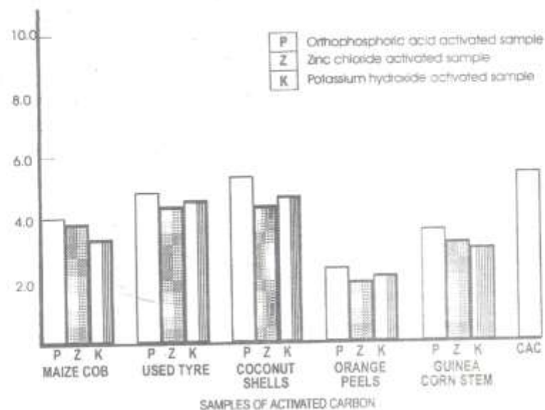
Fig. 2: Adsorption capacity of activated carbon based on decolourisation of methyl red solution
