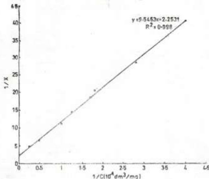
Fig. 10: Langmuir adsorption isotherm of CSK in methylene blue solution.
