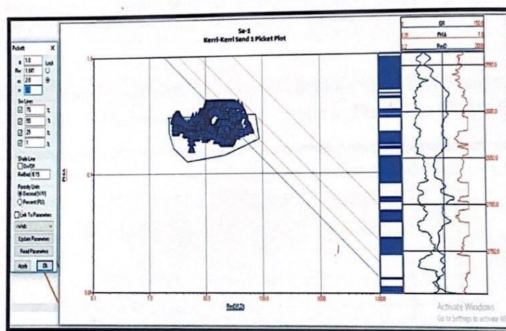
Figure 7: Picket plots of Kerr-Kerri sand-1 in Sa-1 well, R_{wi} is 1.841 \Omega m
