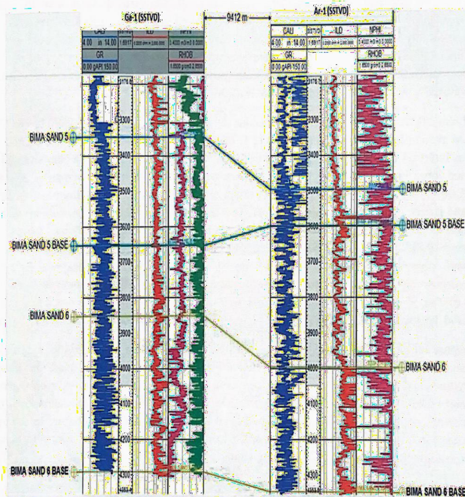
Figure 8: Serrated or Saw Teeth Gamma Ray Motif of Bima Sand, Showing alternation of Shale and Sand Lenses in Ga-1 and Ar-1 wells
