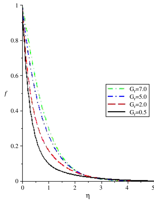
Fig. 4. Velocity profiles for different values of G_r .
