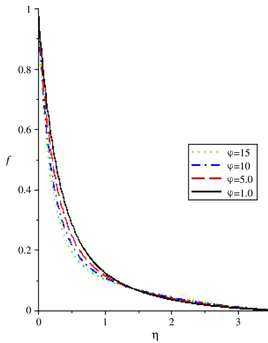
Fig. 6. Velocity profiles for different values of \varphi .
