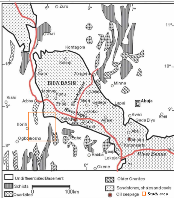
Figure 2: Geological map of Bida Basin and Environs showing the study area (After Obaje, 2011)
