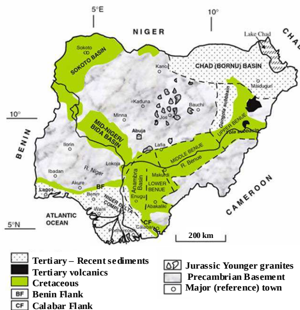
Figure 1: Geological sketch map of Nigeria showing the major geological components (Basement, Younger Granites and Sedimentary basins) and Ilorin, the capital of Kwara state (After Obaje, 2009)
