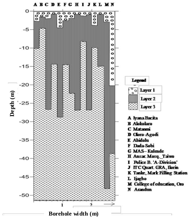
Figure 8 Lithological section of boreholes within the study area (N S)
