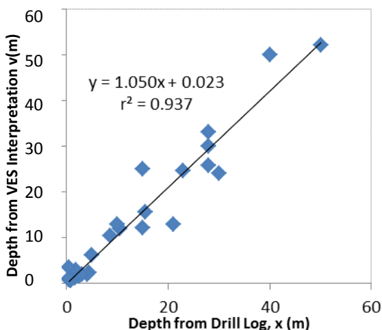
Figure 9: Relationship between VES Interpretation and Drill Log (Regression Analysis)
