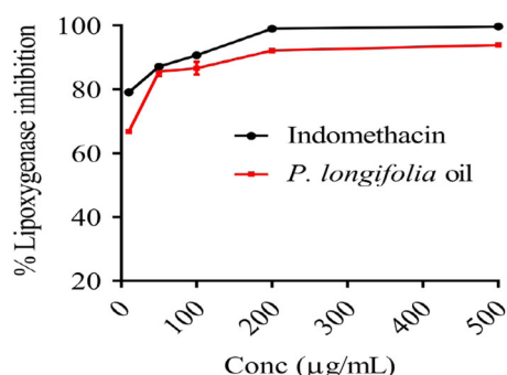
Fig. 1 Lipoxigenase percentage inhibition of Indomethacin (control) and P. longifolia oil
