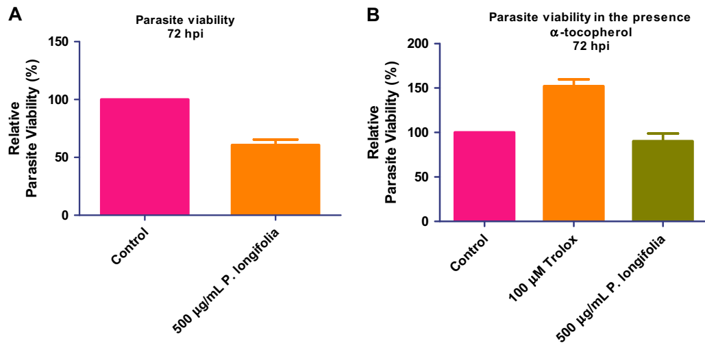
Fig. 5 a-b Anti- T. gondii potential of P. longifolia in the absence/presence of \alpha -tocopherol (trolox). The experiment was conducted independently thrice and in triplicates
