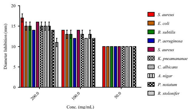
Fig. 4 Comparison anti-microbial activities of P. longifolia oil against the tested organisms
