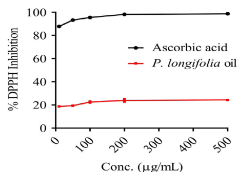
Fig. 2 DPPH anti-oxidant activities of ascorbic acid (control) and P. longifolia seed oil
