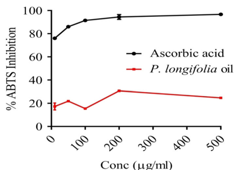
Fig. 3 ABTS percentage inhibition of ascorbic acid (control) and P. longifolia oil
