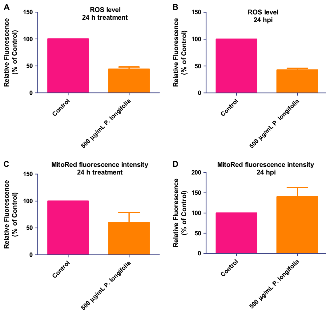
Fig. 6 a-d ROS level and mitoRed fluorescence intensity following 24 h treatment with P. longifolia ; a without T. gondii infection; b with T. gondii infection; c without T. gondii infection; d with T. gondii infection. The experiment was conducted independently thrice and in triplicates
