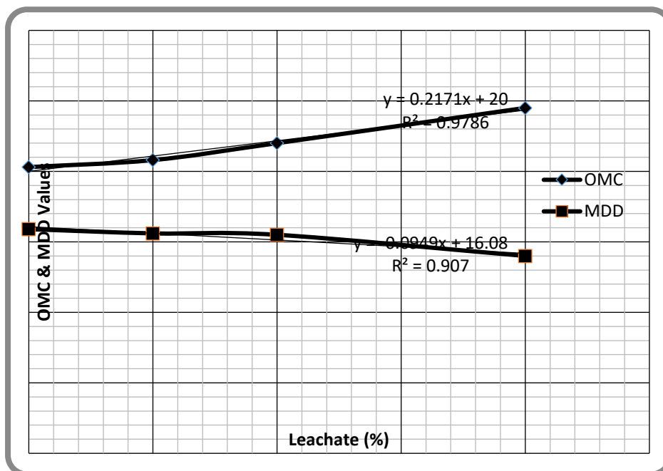
Fig. 3: Relationship between compaction parameters and Leachate content.
