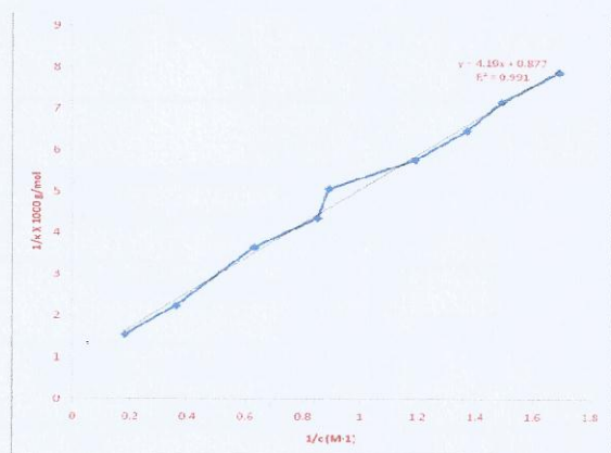
Figure 1: Langmuir isotherm of plot of adsorption of acetic acid on activated carbon from Jatropha curcas shell
