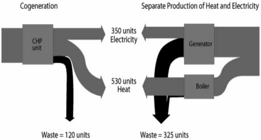
Figure 4. Cogeneration of Heat and Power (image courtesy of WADE)
